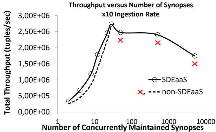
Figure 13: Comparison of SDAaaS vs non-SDEaaS. x signs denote that non-SDEaaS cannot maintain more than 40 synopses simultaneously since available task slots are depleted.
