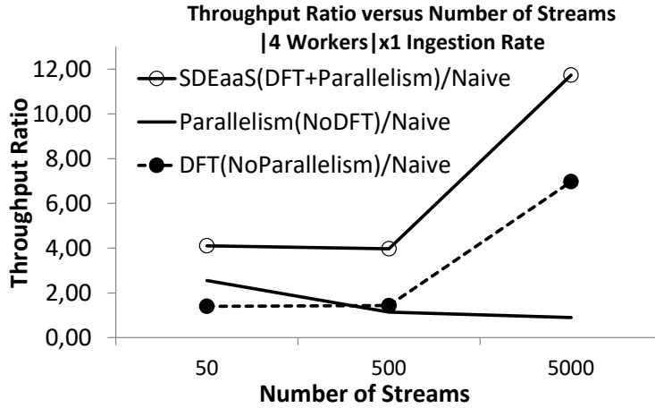
Figure 11: Comparative Analysis in Executing the Workflow of Figure 6 using SDE.DFT.
