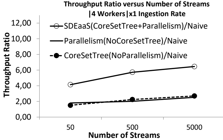
Figure 12: Comparative Analysis in Executing the Workflow of Figure 6 using SDE. CoreSetTree.
