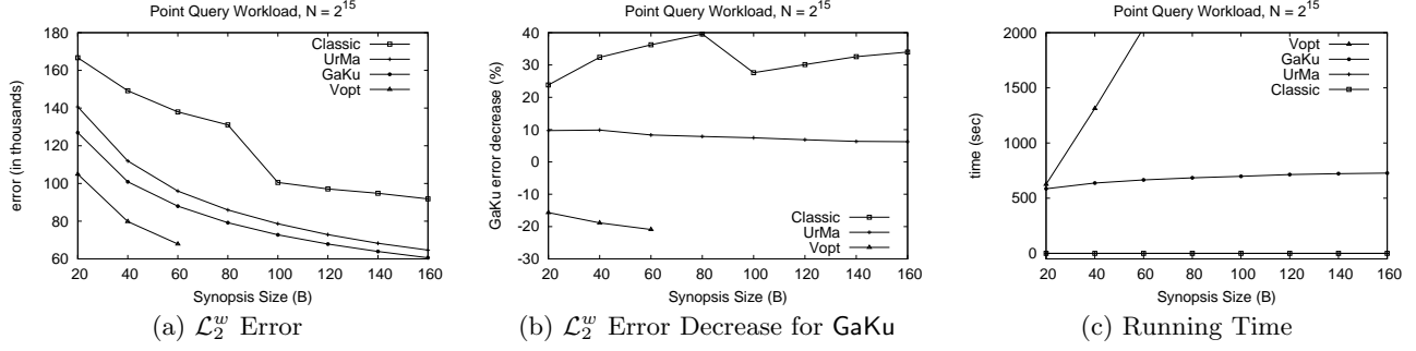
Figure 2: Accuracy and Running Time vs. Synopsis Size (B) for Point Query Workloads
