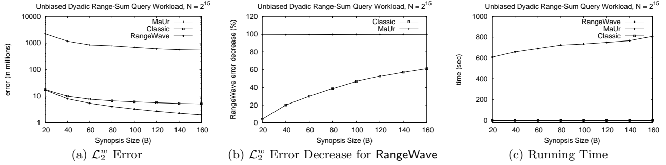
Figure 4: Accuracy and Running Time vs. Synopsis Size (B) for Unbiased Dyadic Range-Sum Query Workload
