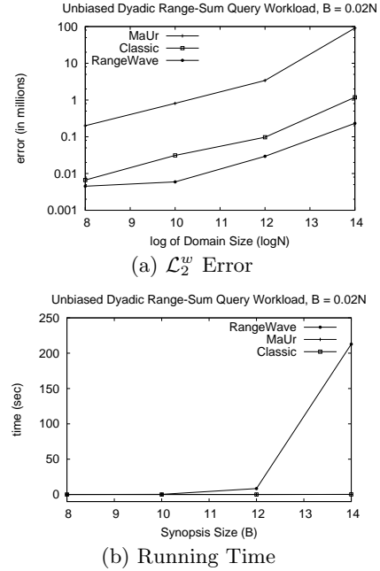
Figure 5: Accuracy and Running Time vs. Domain Size (N) for Unbiased Dyadic Range-Sum Query Workload
