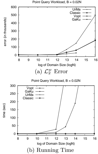
Figure 3: Accuracy and Running Time vs. Domain Size (N) for Point Query Workloads
