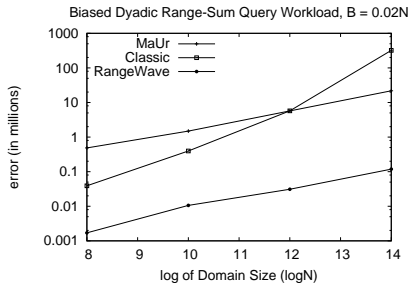
Figure 7: Accuracy vs. Domain Size (N) for Biased Dyadic Range-Sum Query Workload
