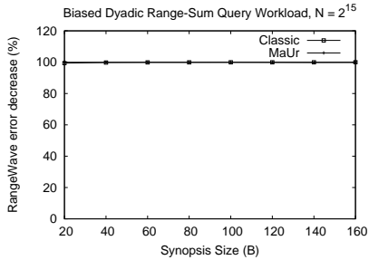
(b) L_2^w Error Decrease for RangeWave
