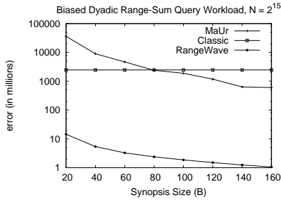
(a) L_2^w Error
